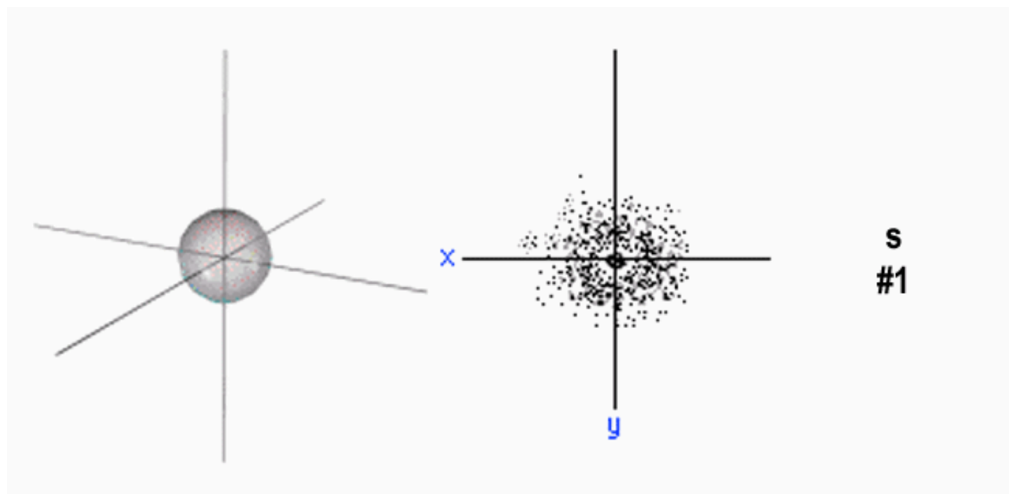
Figure 6-12. Probability density plots of some hydrogen atomic orbitals. The density of the dots represents the probability of finding the electron in that region.
