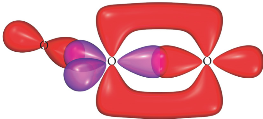
Valence bond model
