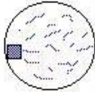
Gamma ray
