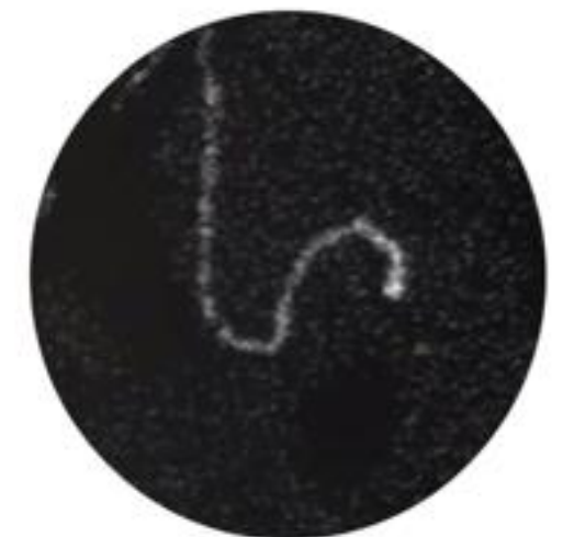
Beta particle
