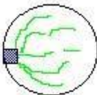
Beta particle
