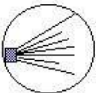
Alpha particle
